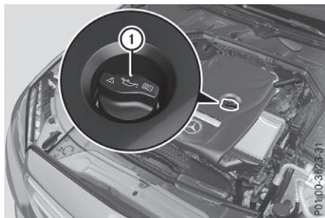
Top up the engine oil (example)
