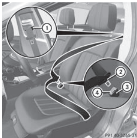
CLS Shooting Brake (example)
